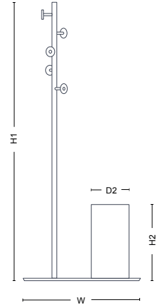
Double Coat Rack + Umbrella Stand H: 1800 mm, 70.9" H2: 480 mm, 18.9" D2: D240 mm, D9.4" W: 760 mm, 29.9" D: 420 mm, 16.5"
