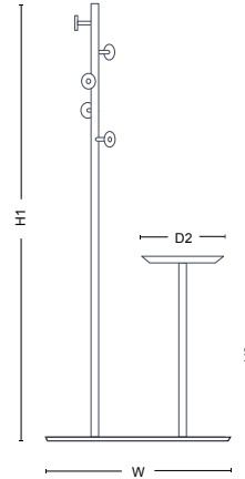
Double Coat Rack + Side Table H: 1800 mm, 70.9" H2: 760 mm, 29.9" D2: D320 mm, D12.6" W: 760 mm, 29.9" D: 420 mm, 16.5"
